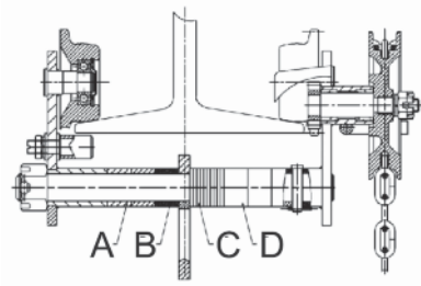
Geared Trolley Do 191/T
